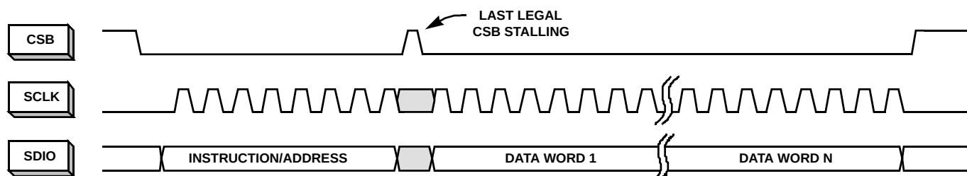
FIGURE 57. N-BYTE TRANSFER
