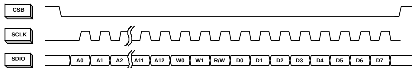
FIGURE 53. LSB-FIRST ADDRESSING
