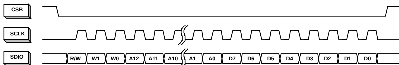
FIGURE 52. MSB-FIRST ADDRESSING
