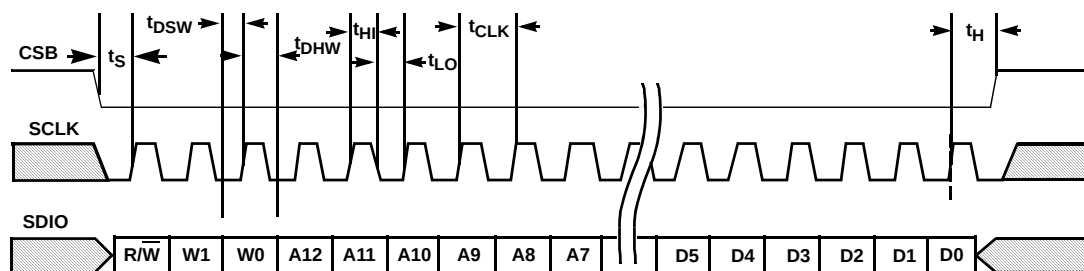
FIGURE 54. SPI WRITE
