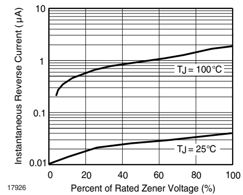
Figure 5. Typical Reverse Characteristics
