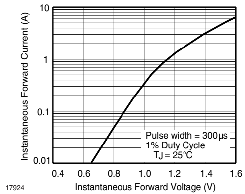
Figure 4. Typical Instantaneous Forward Characteristics for SML4763
