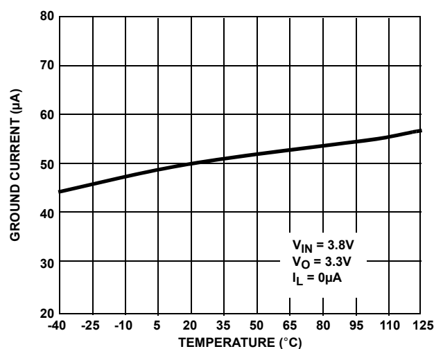
FIGURE 12. GROUND CURRENT vs TEMPERATURE
