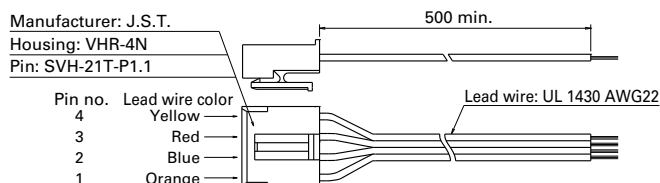
Motor cable Bipolar model no.: 4837961-1
