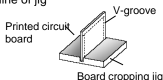
Board cropping jig
