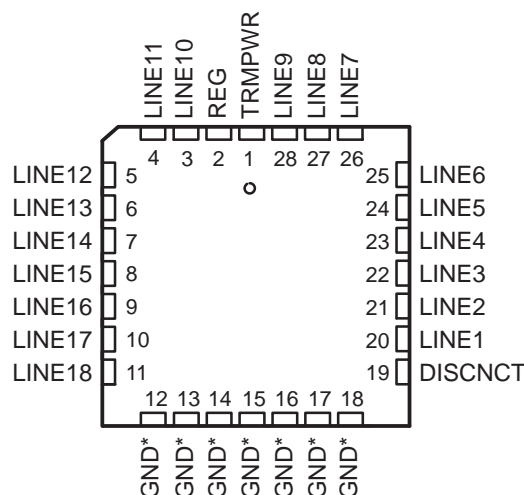
QP PACKAGE TOP VIEW
