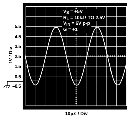
Figure 31. Output Voltage
