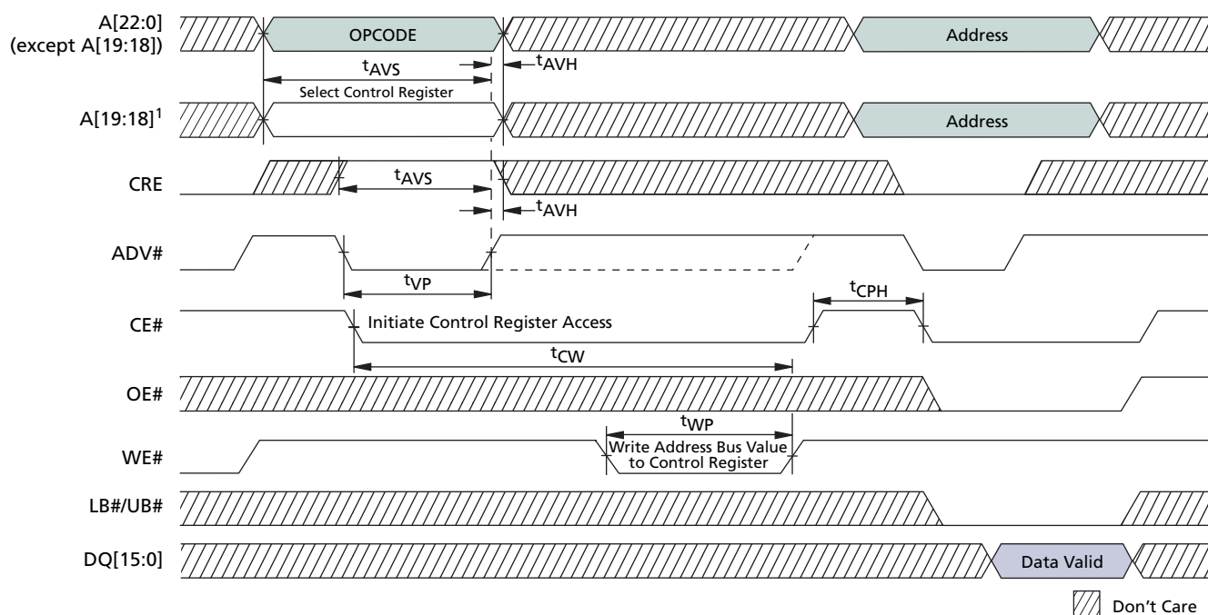
Figure 12: Configuration Register WRITE, Asynchronous Mode, Followed by READ ARRAY Operation
