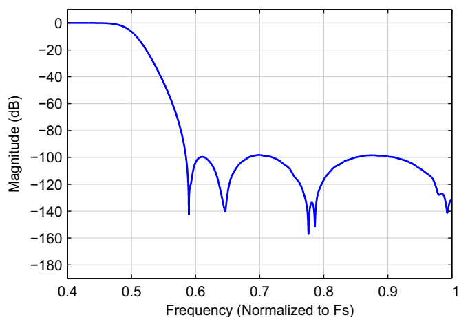
Figure 9-2. Stopband Attenuation
