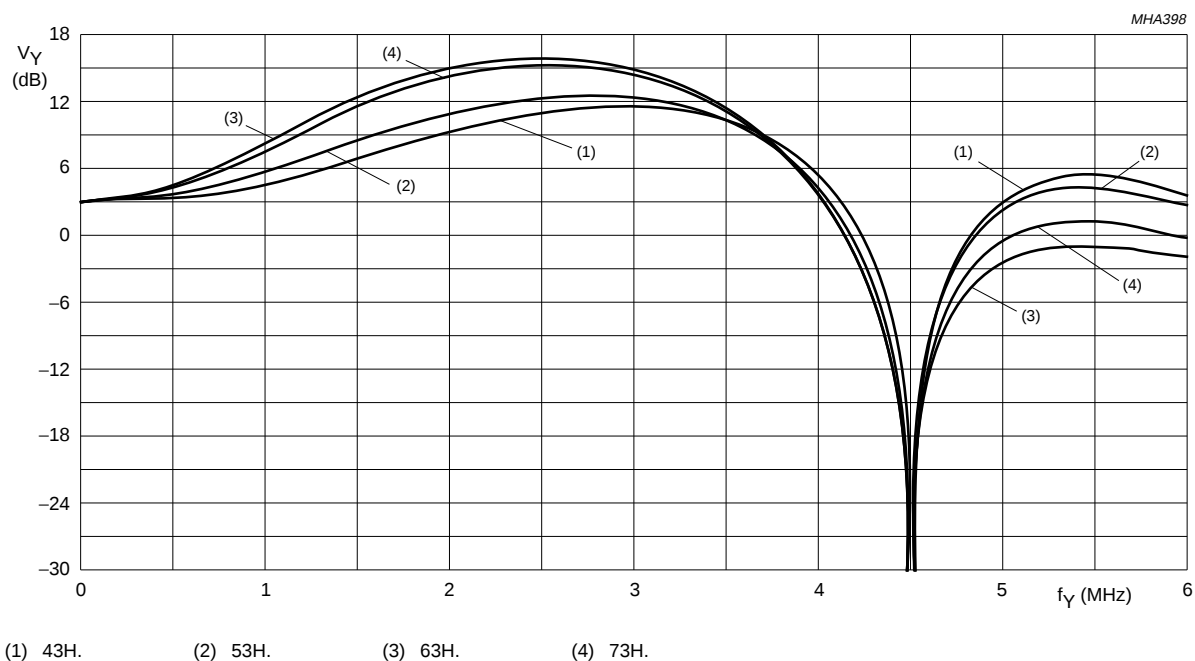
Fig.19 Luminance control in 50 Hz/CVBS mode controllable by subaddress byte 06; pre-filter on and coring off; maximum aperture band-pass filter characteristic.
