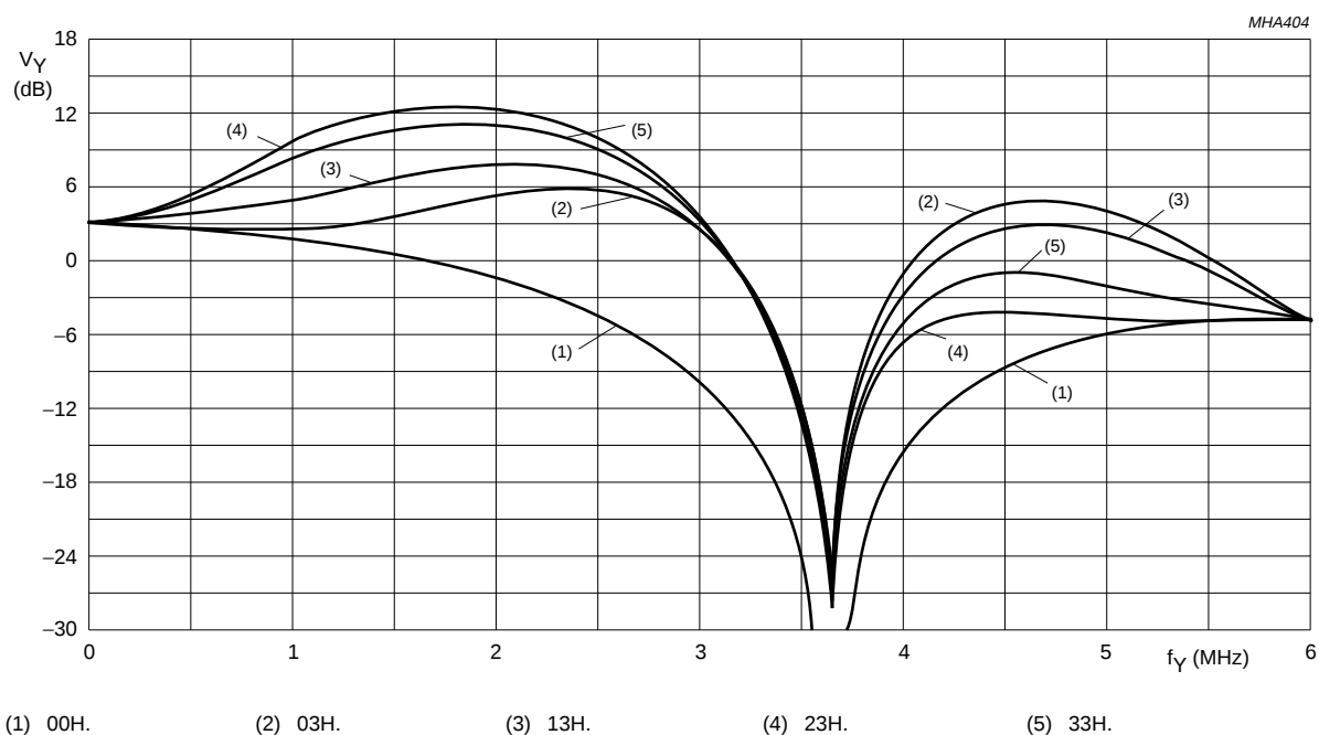
Fig.24 Luminance control in 60 Hz/CVBS mode controllable by subaddress byte 06; pre-filter off and coring off; maximum and minimum aperture band-pass filter characteristics.
