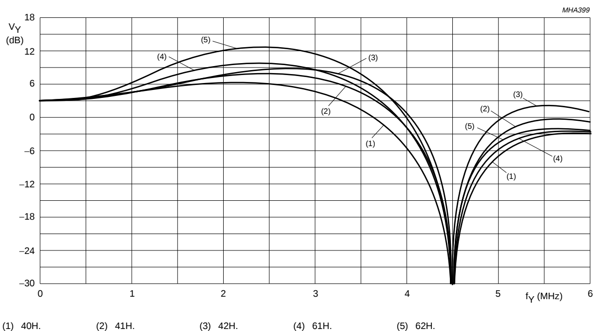
Fig.20 Luminance control in 50 Hz/CVBS mode controllable by subaddress byte 06; pre-filter on and coring off; other aperture band-pass filter characteristic.
