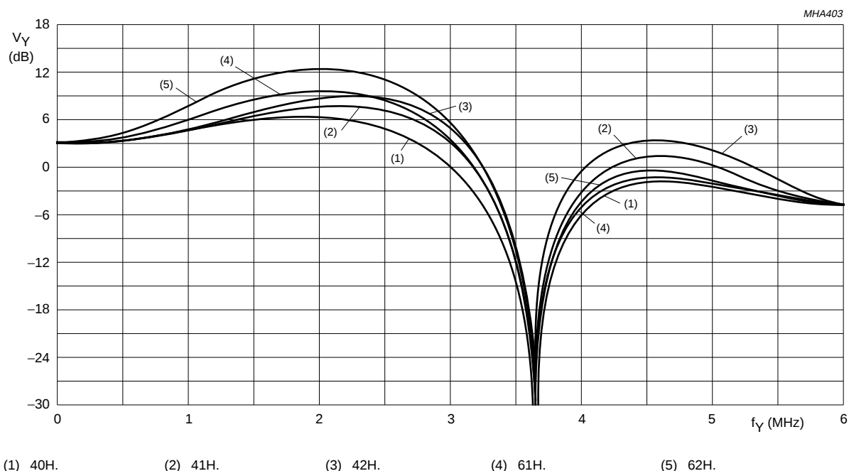
Fig.23 Luminance control in 60 Hz/CVBS mode controllable by subaddress byte 06; pre-filter on and coring off; other aperture band-pass filter characteristics.
