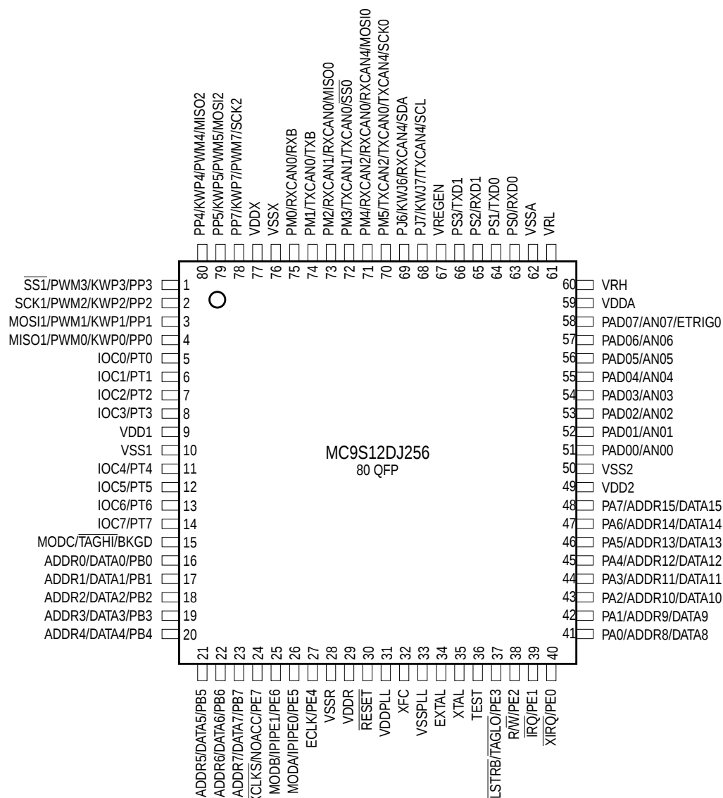
Figure 2-3 Pin Assignments in 80-pin QFP for MC9S12DJ256
