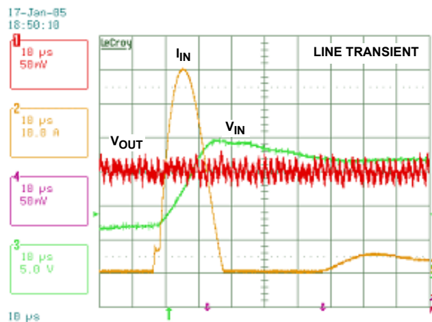
FIGURE 12. 8V-20V INPUT LINE TRANSIENT RESPONSE, C_{IN} = 240\mu F
