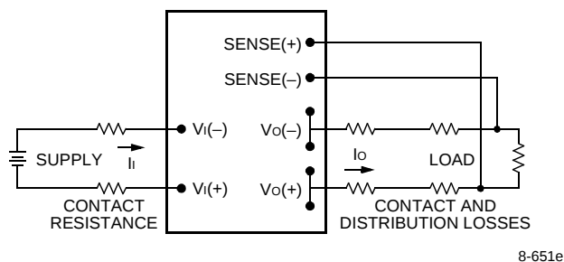
Figure 16. Effective Circuit Configuration for Single-Module Remote-Sense Operation
