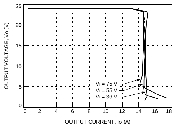
Figure 4. Typical FW300H1 Output Characteristics at Room Temperature
