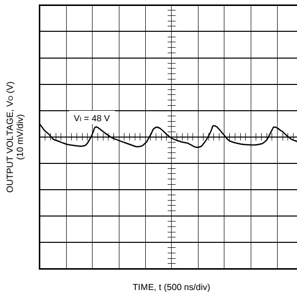
Figure 7. Typical FW250H1 Output Ripple Voltage at Room Temperature and 50 A Output
