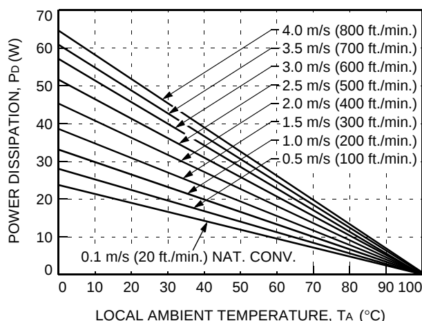
Figure 22. Convection Power Derating with No Heat Sink; Airflow Along Length (Longitudinal)
