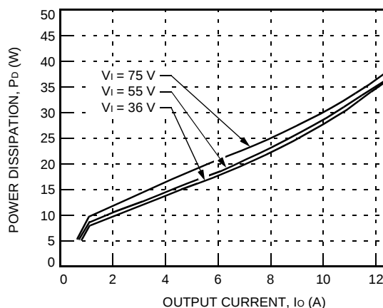
Figure 26. FW300H1 Power Dissipation vs. Output Current
