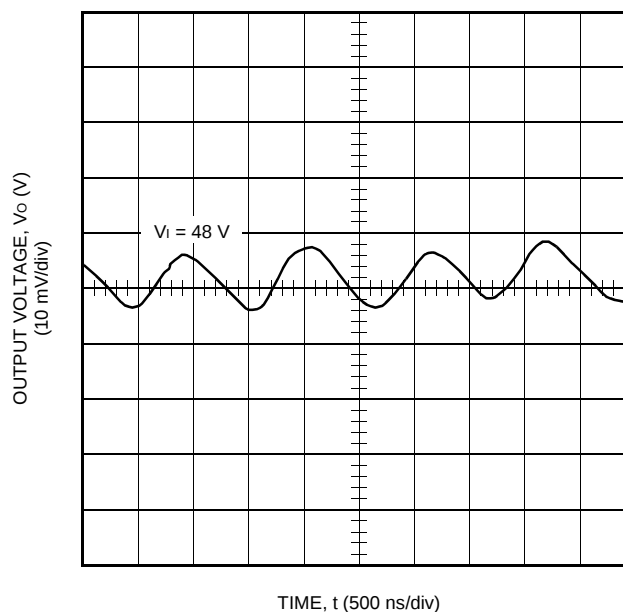
Figure 8. Typical FW300H1 Output Ripple Voltage at Room Temperature and 60 A Output
