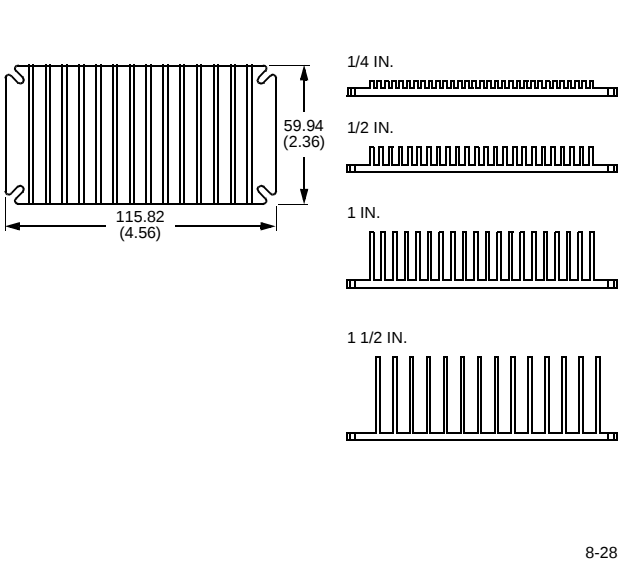
Figure 29. Transverse Heat Sink
