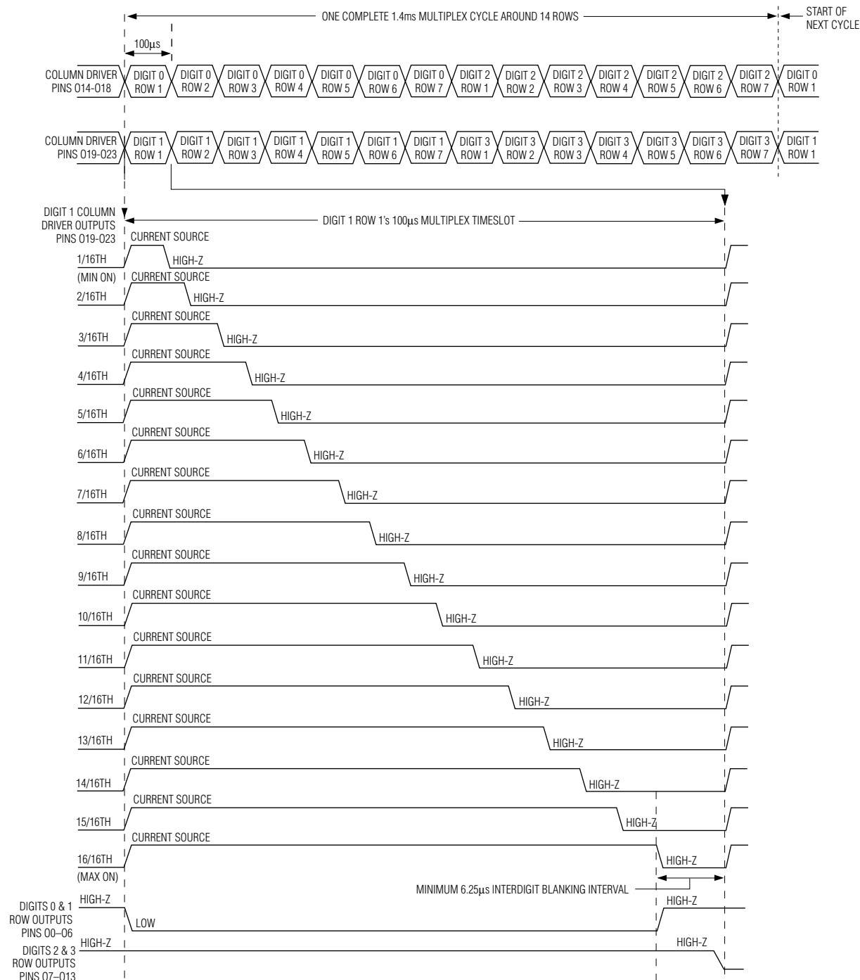
Figure 7. Multiplex Timing Diagram (OSC = 4MHz)
