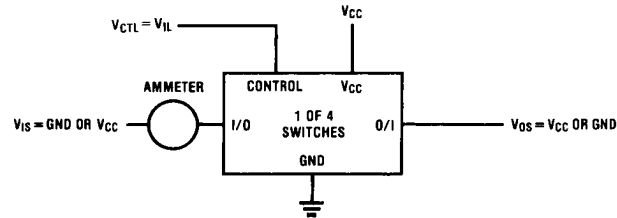
FIGURE 3. "OFF" Channel Leakage Current
