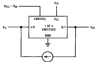
FIGURE 1. "ON" Resistance
