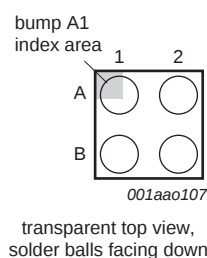
Fig 2. Pin configuration for WLCSP4
