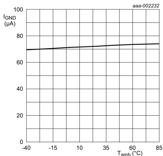
Fig 11. Quiescent current for LD6836CX4/25H
