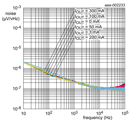
Fig 12. Noise density for LD6836x/25x
