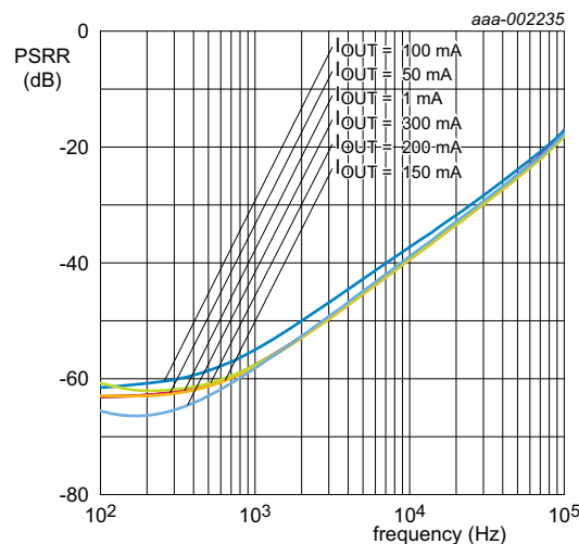
Fig 6. PSRR of LD6836TD/25H
