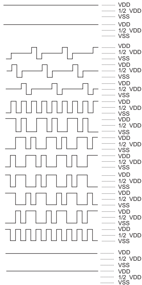
LCD driver output (1/3 duty, 1/2 bias)
