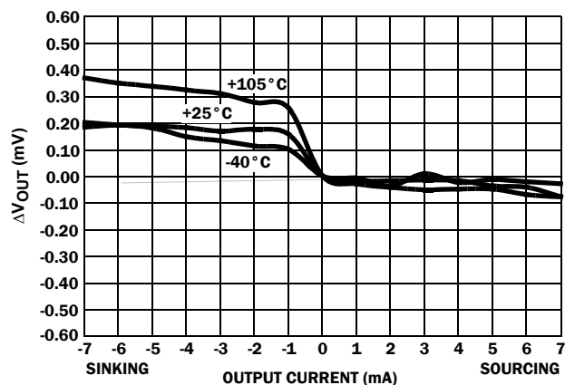
FIGURE 106. LOAD REGULATION
