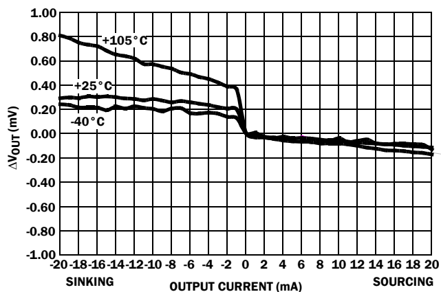
FIGURE 107. LOAD REGULATION OVER-TEMPERATURE
