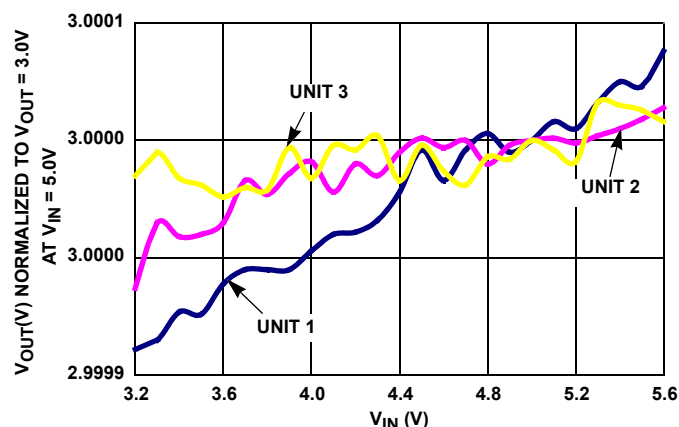
FIGURE 86. LINE REGULATION (3 REPRESENTATIVE UNITS)
