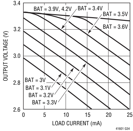
3.3V LDO Output Voltage vs Load Current, V_{\text{BUS}} = 0\text{V}
