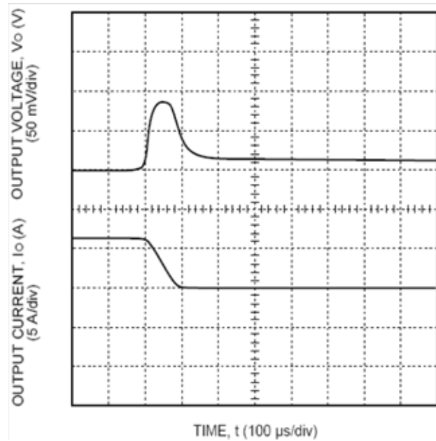
Figure 11. Typical Transient response to Step load change from 100% to 0% of I_{O,max} at 5V Input. (Waveform Averaged to remove ripple)
