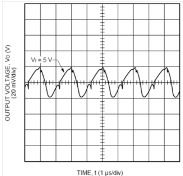
Figure 7. Typical Output Ripple Voltage for NH020M (6A Output Current).
