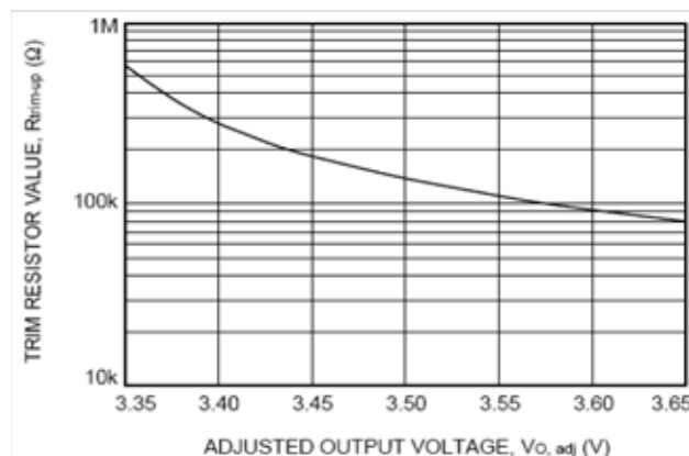
Figure 26. NH020F Rtrim-up Test Results .
