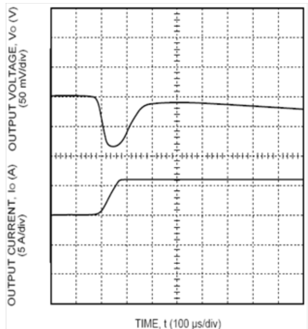
Figure 10. Typical Transient response to Step load change from 0% to 100% of I_{0,\text{max}} at 5V Input .
