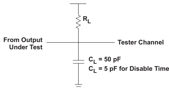
Figure 12. Test Load Circuit for AC Timing Measurements
