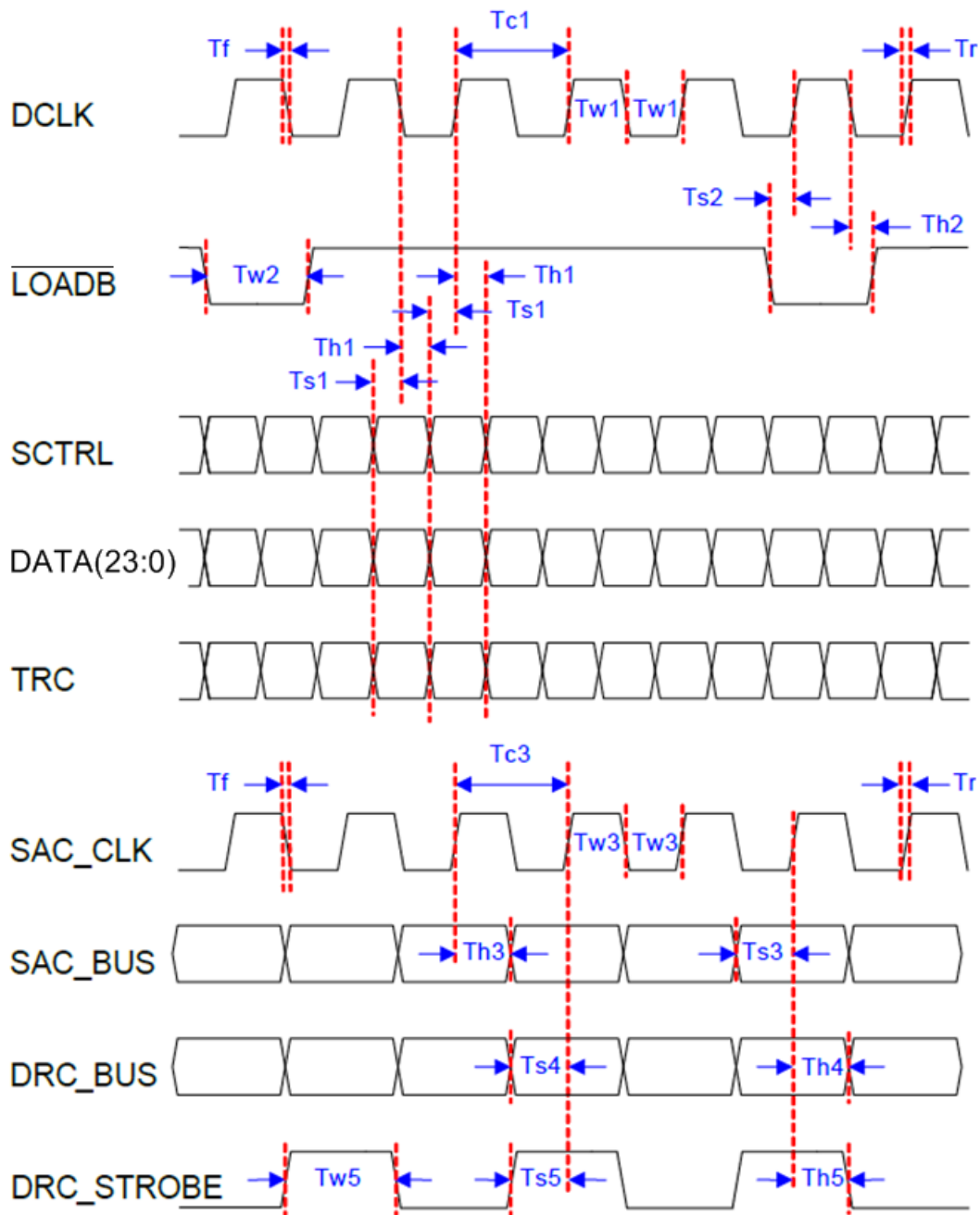
Figure 13. Switching Characteristics
