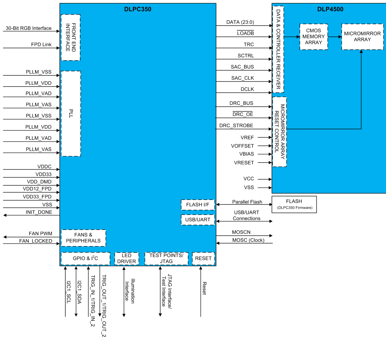
Figure 1. DLP 0.45 WXGA Chip Set
