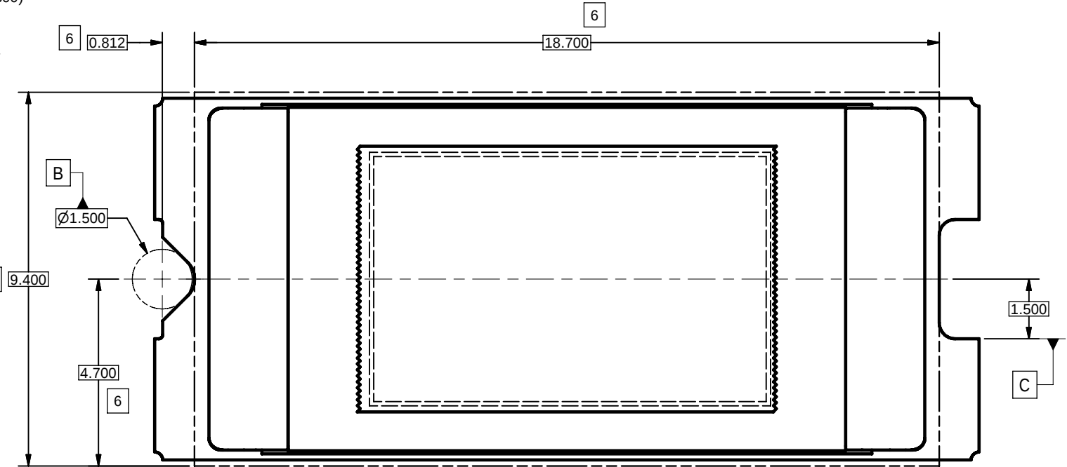
VIEW C ENCAPSULANT MAXIMUM X/Y DIMENSIONS SCALE 15 : 1 (FROM SHEET 1)
