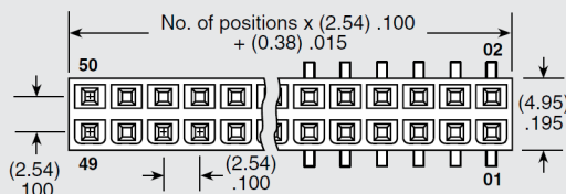
Through-hole
