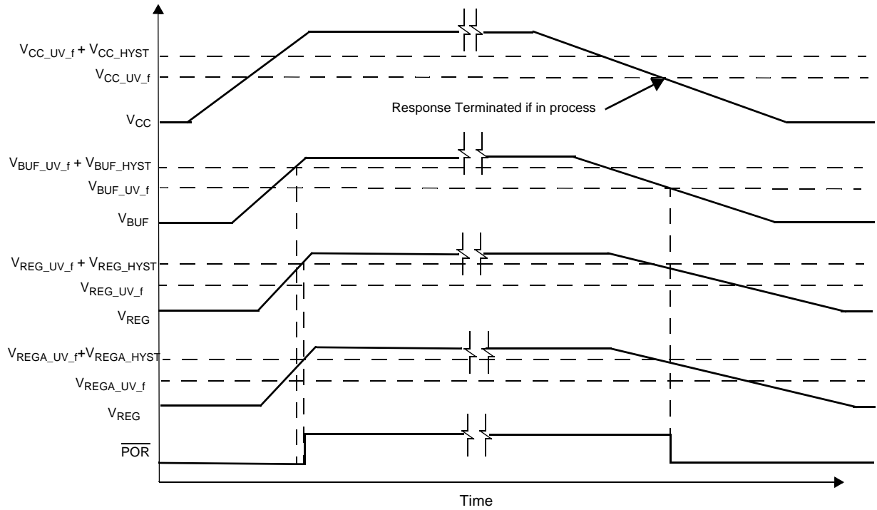
Figure 7. Powerup Timing
