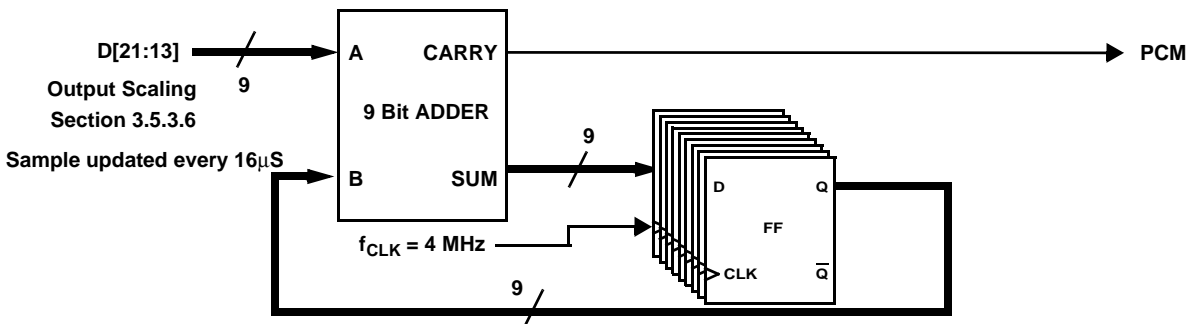
Figure 24. PCM Output Function Block Diagram
