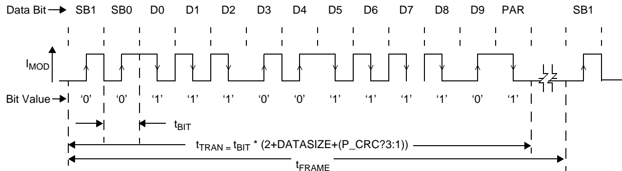
Figure 31. Example Manchester Encoded Data Transfer - PSI5-x10P
