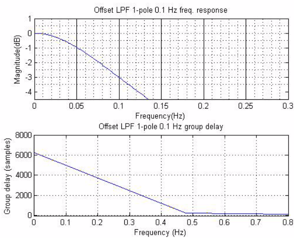
Figure 22. 0.1 Hz Offset Cancellation Low-Pass Filter Characteristics
