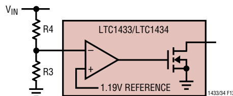
Figure 12. Low-Battery Comparator
