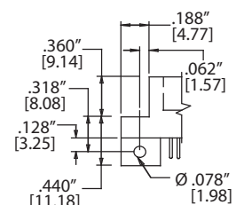
STRADDLE MOUNT (Q)
