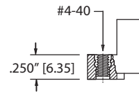
FLUSH MOUNTING WITH THREADED INSERT (T)
