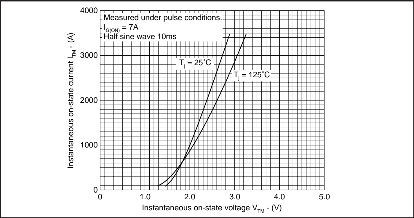
Fig.2 On-state characteristics
