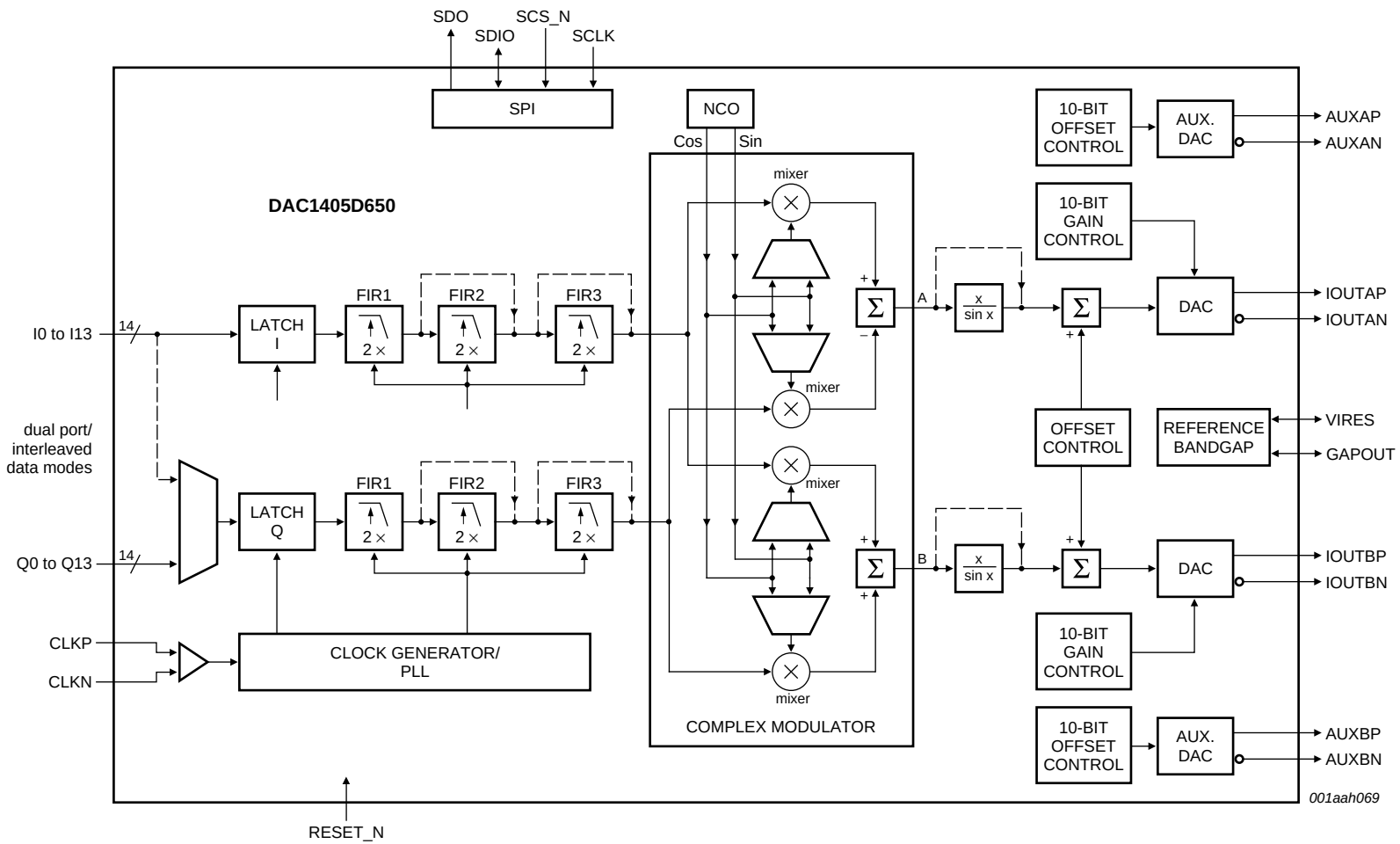
Fig 1. Block diagram
