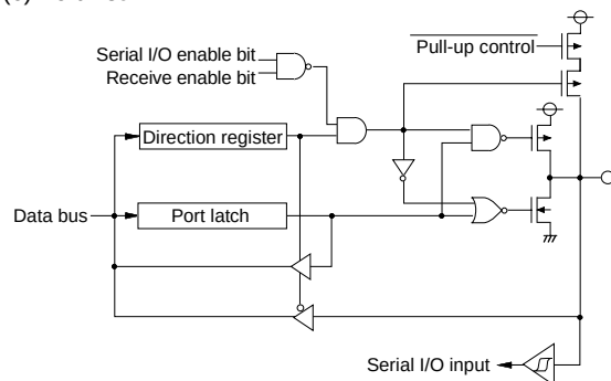
(6) Port P33
