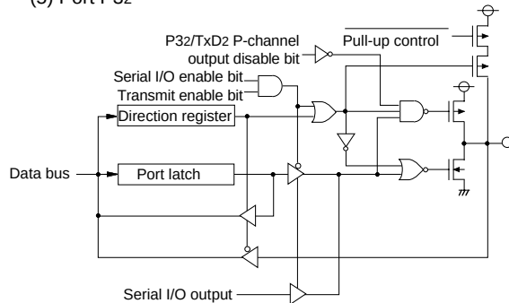
(5) Port P32
