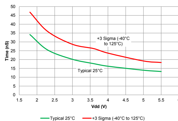
Figure 41-57. I/O Rise Time, Slew Rate Control Enabled
