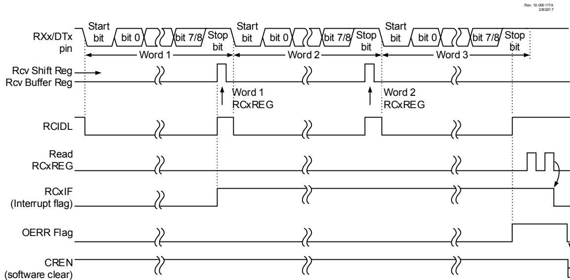
Figure 29-5. Asynchronous Reception
