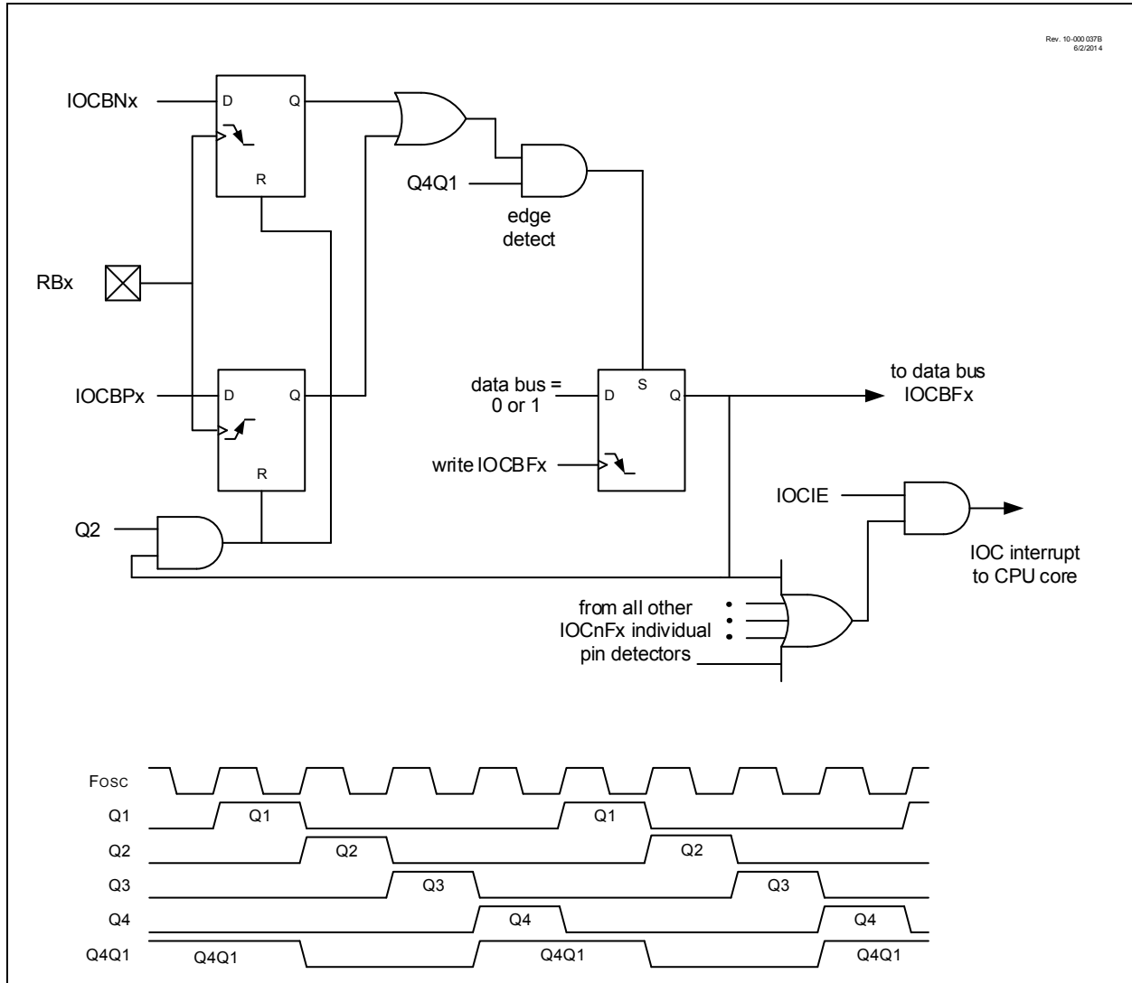
Figure 16-1. Interrupt-on-Change Block Diagram (PORTB Example)
