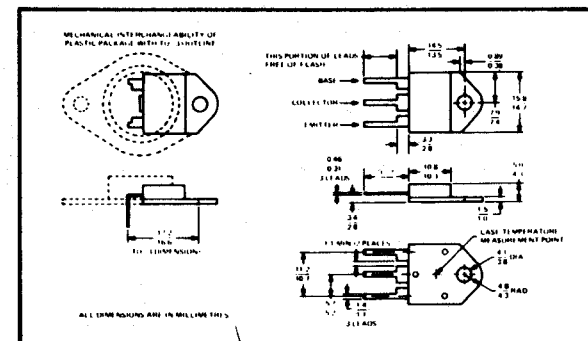
TO-3 Plastic
