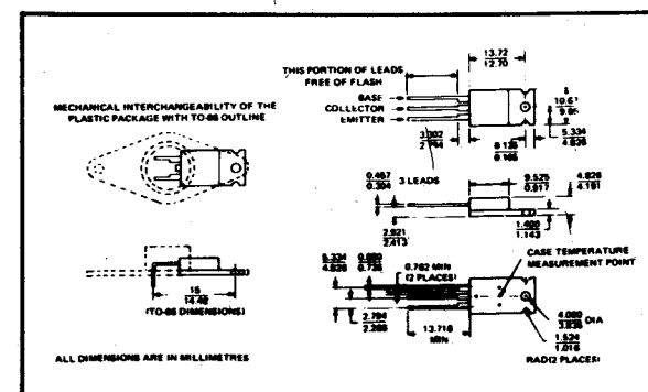
TO-220AB Plastic
