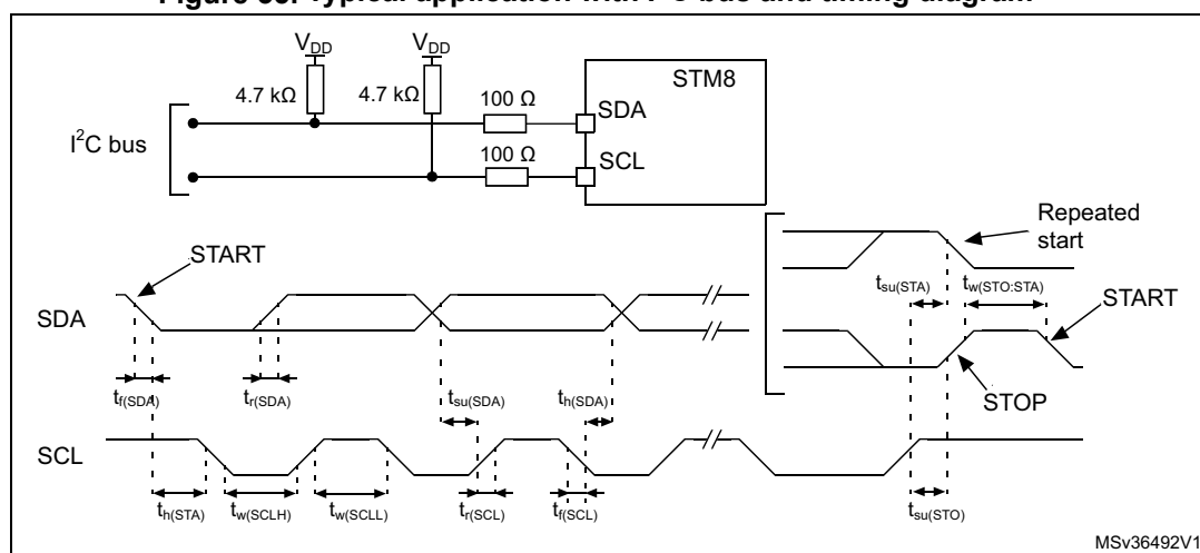
Figure 35. Typical application with I 2 C bus and timing diagram (1)
