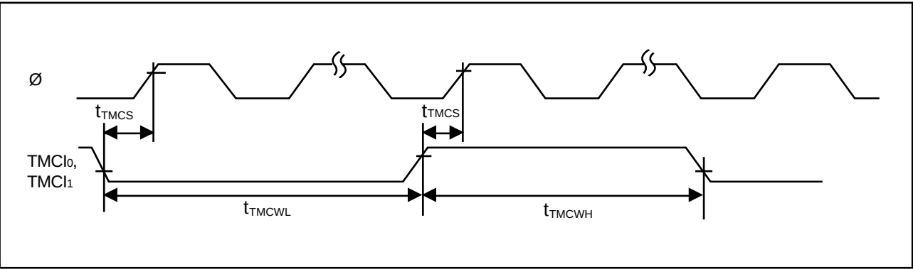
Figure 17-14. 8-Bit Timer Clock Input Timing
