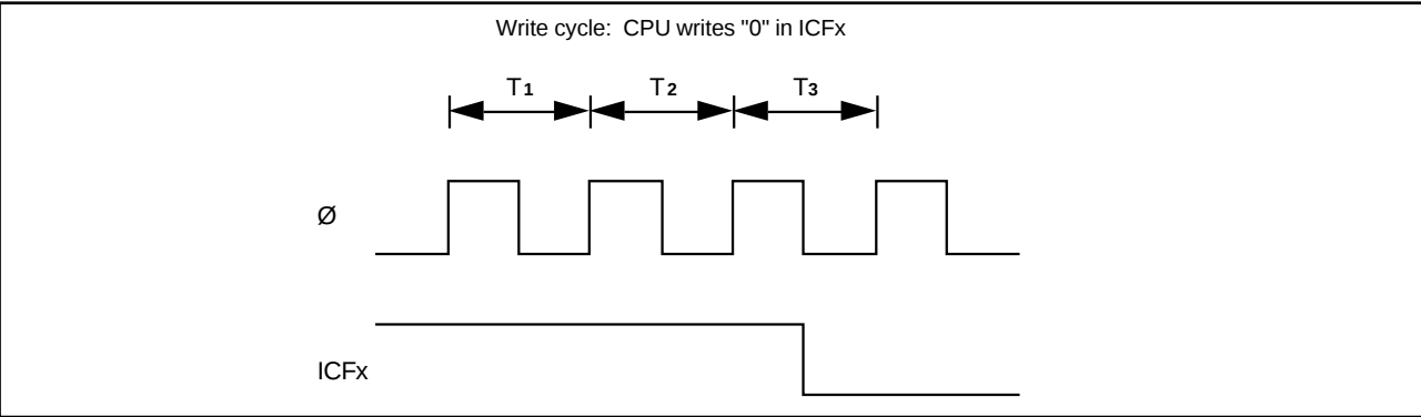
Figure 6-17. Clearing of Input Capture Flag
