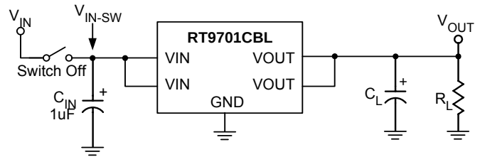
Test Circuit 2
