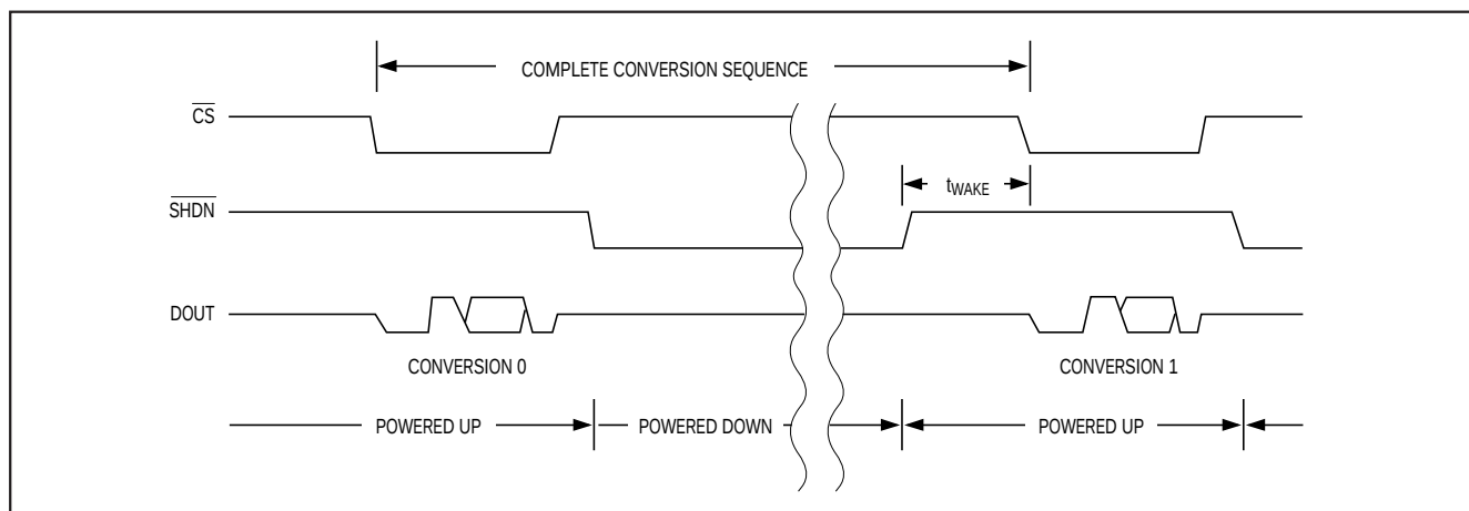
Figure 5. Shutdown Sequence
