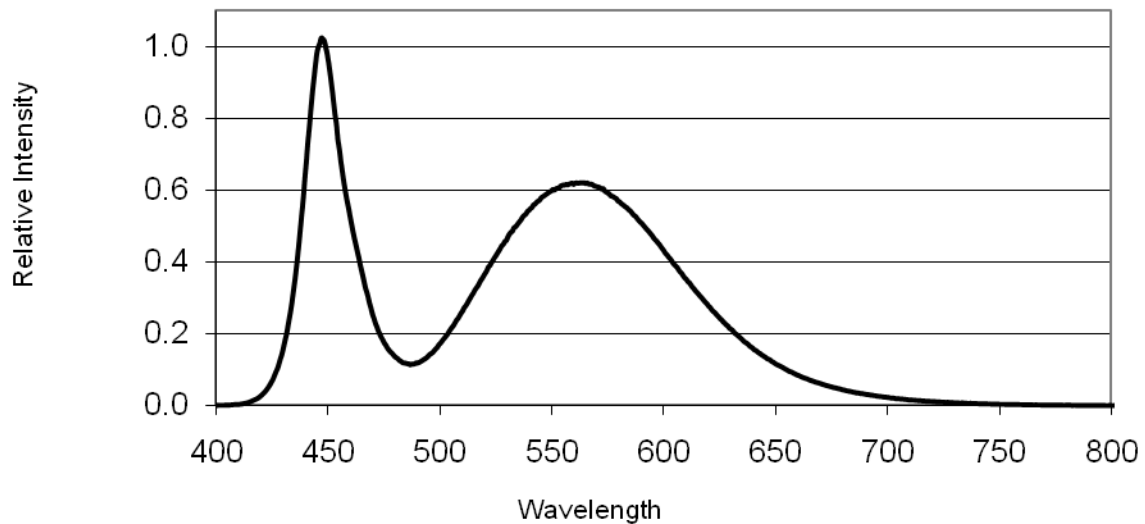
Figure 5: Typical Cool White Color Spectrum
