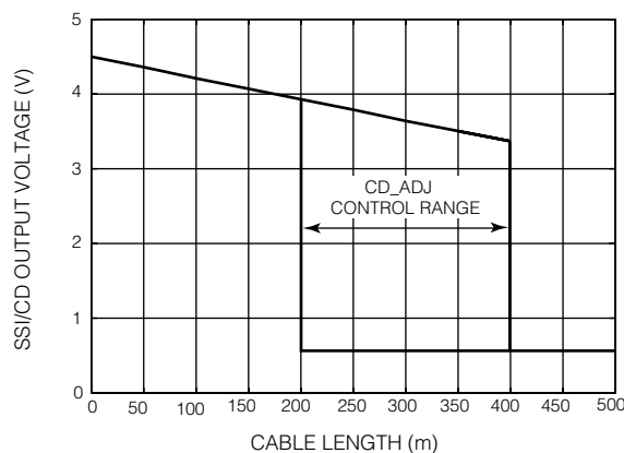
Fig. 16 SSI/CD Voltage vs. Cable Length
