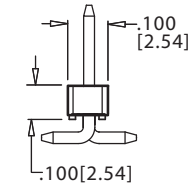
SMT, -M30 Modification Code
