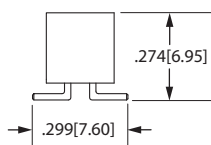
SURFACE MOUNT (SM) Example P/N: SBH21-NBPN-D20-SM-BK
