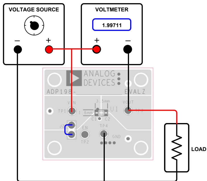
Figure 7. WLCSP R_{DS(on)} Measurement
