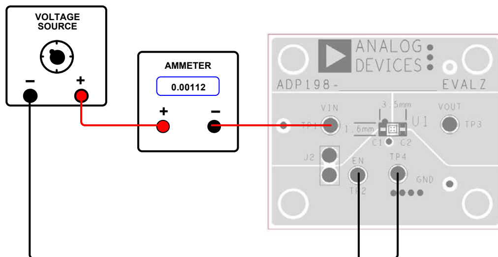
Figure 13. WLCSP Shutdown Current Measurement
