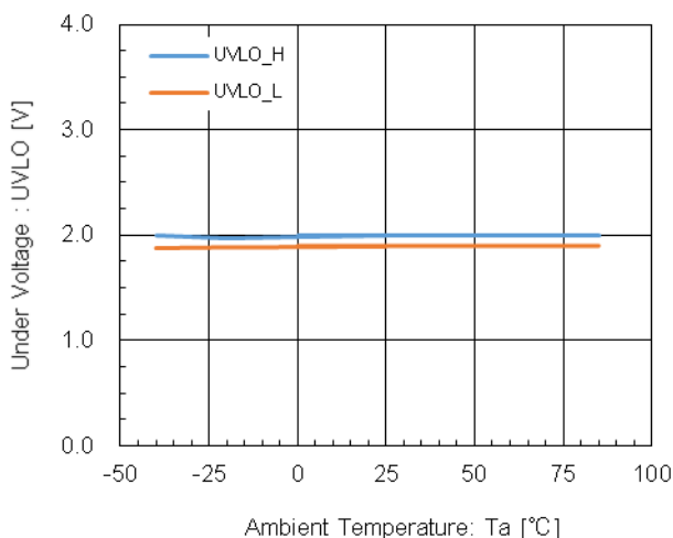
(7) UVLO Voltage vs. Ambient Temperature
