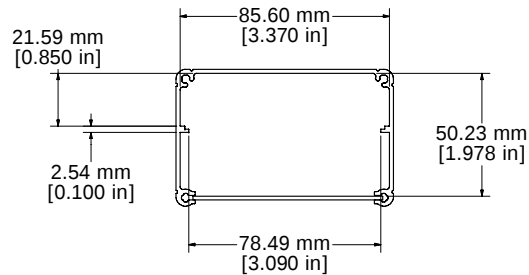
EXTRUSION - INSIDE
