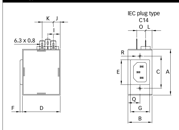
1 to 15 A types
