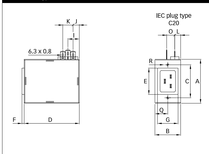
16 and 20 A types
