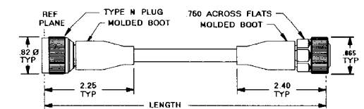
TS1878 CONFIGURATION
