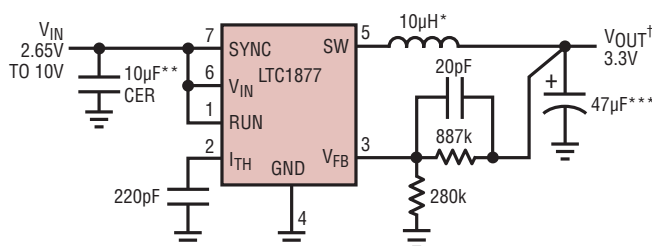
High Efficiency Step-Down Converter
