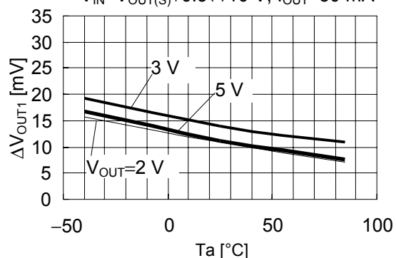
S-814A20A/S-814A30A/S-814A50A
