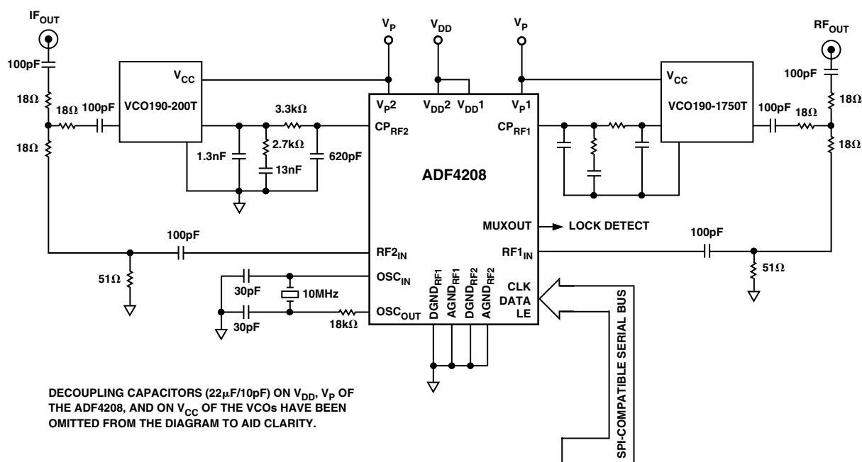
Figure 8. Local Oscillator for WCDMA Receiver Using the ADF4208
