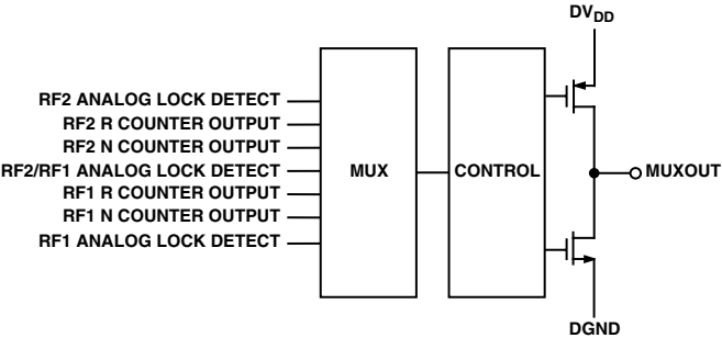
Figure 6. MUXOUT Circuit
