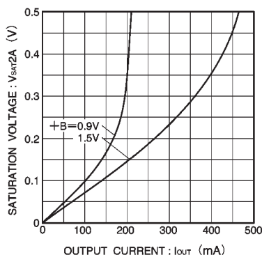
Fig.9 Speaker control unit (loud volume) : saturation voltage vs. output current
