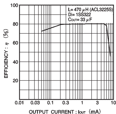
Fig.6 DC / DC converter unit efficiency vs. load current
