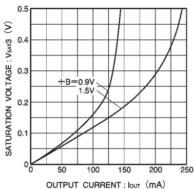
Fig.13 LED control unit: saturation voltage vs. output current
