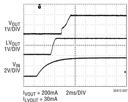
Output (Auto-Start-Up Sequence) vs Time
