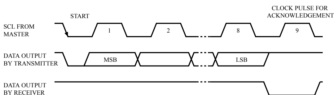
Figure 12. Acknowledgement sequence
