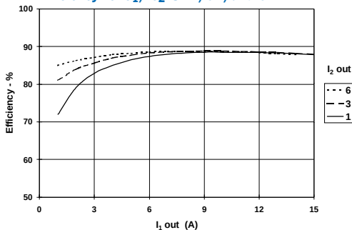
Efficiency vs I_{O1} ; I_{O2} @1A, 3A, and 6A
