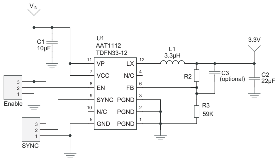
Figure 1: AAT1112 Schematic.
